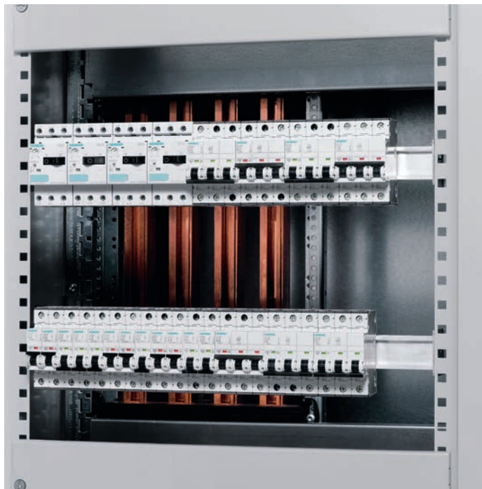
The multi-profile busbar allows for easy mounting of modular installation devices
