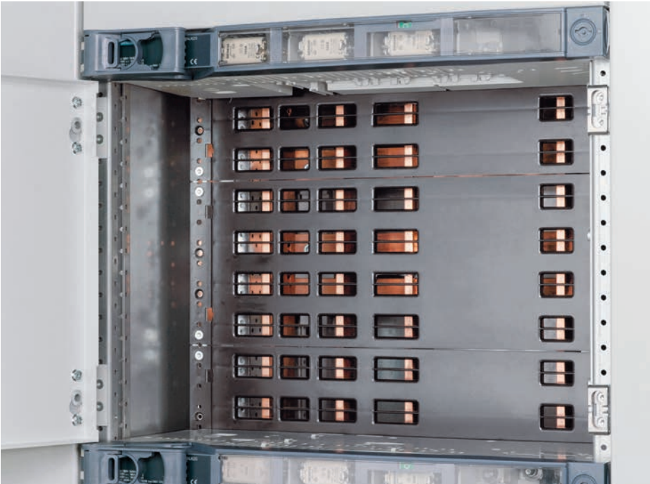
Plug-in busbar system, with test finger safety cover
