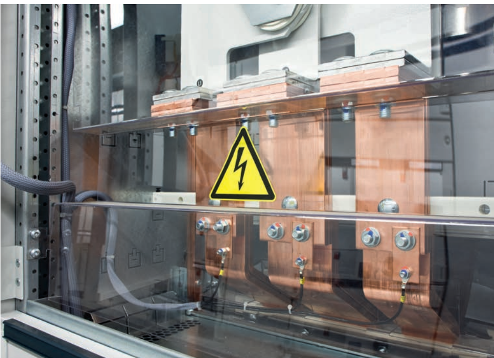
Continuous power supply by means of design verified connection to SIVACON 8PS busbar trunking systems
